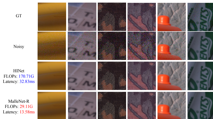
Fig. 4. Randomly picked testing patches from MalleNet and previous state-of-the-art methods on real-world noise benchmark (SIDDD [1]). Best viewed in color and zoomed in.
